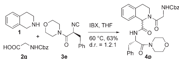
Scheme 3. Three-component reaction to synthesize a tetrahydroisoquinoline-containing tripeptide.
